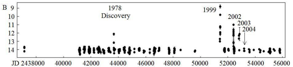
Figure 1. Historical half-century light curve of V4641 Sgr
