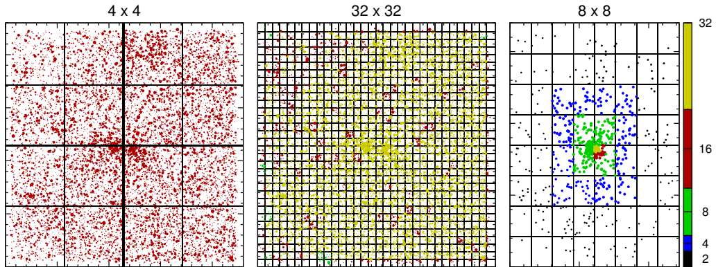
Figure 1: Astrometric calibration in sub-fields. Left : Dividing source list into 4-by-4 sub-fields (recursion depth 2). Middle : The result of recursive refinement of source astrometry. The final recursion depth is shown with colors. Right : Astrometry for a non-square plate with higher density of sources in the center.
