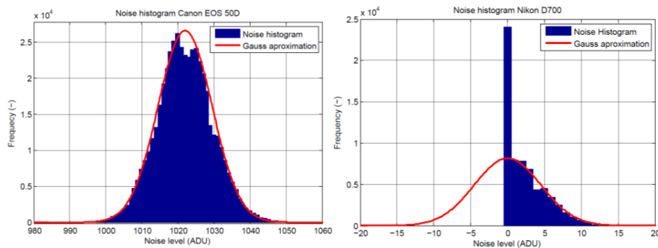
Fig. 4. Bias noise for Canon 50D and Nikon D700
