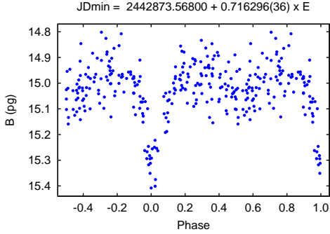
Figure 4: Lightcurve of B1.0 0953-0319502.
