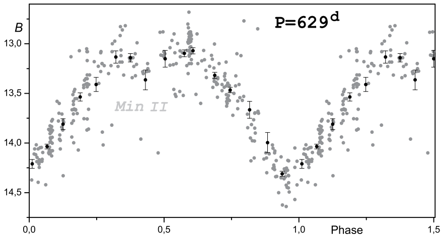
Figure 3: The phase light curve of FG Ser.
