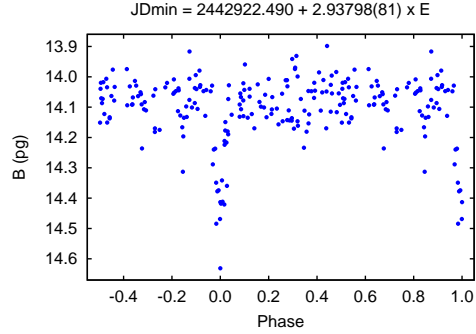
Figure 5: Lightcurve of B1.0 0944-0313124.
