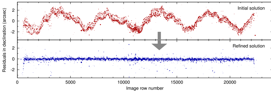
Figure 2: Astrometric residuals after initial solution and after refined calibration in sub-fields. The ripples, caused by a flatbed scanner, disappear after refinement.
