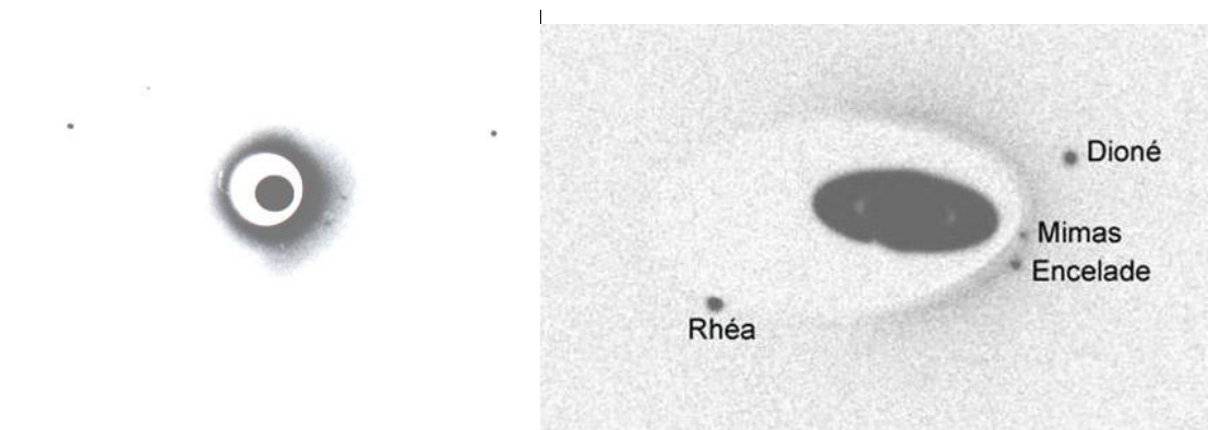
Left : the planet Mars (under a metallic filter) surrounded by light diffusion in which the satellites are visible. Farther are the stars referenced in the UCAC2 catalogue. [4] At right, the Saturnian system with the planet Saturn under a metallic filter.
